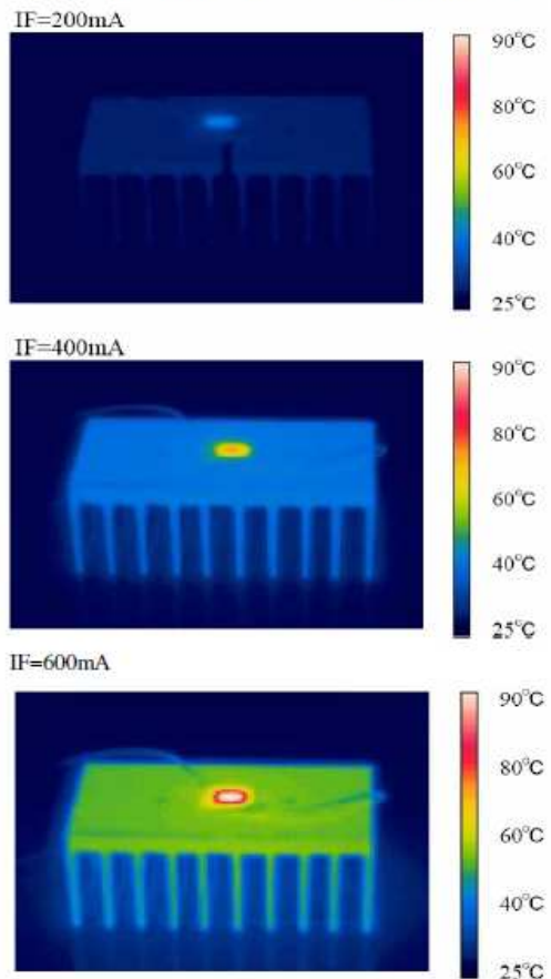
<Fig.3> Board B (surface area=20,600mm 2 )
