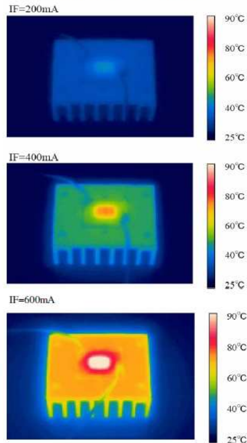
<Fig.2> Board A (surface area=10,300mm 2 )
