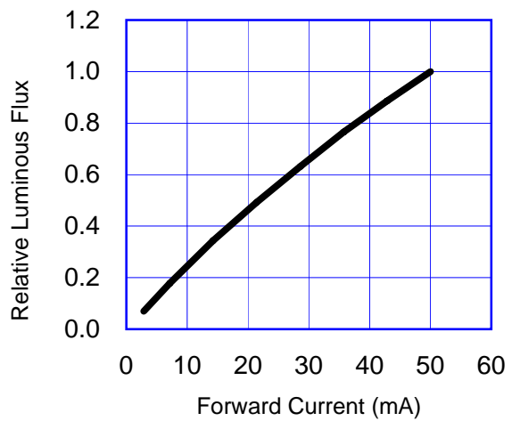
Fig 2. Relative Luminous Flux vs. Forward Current for White, Warm White at T_j=25^\circ\text{C} maintained.
