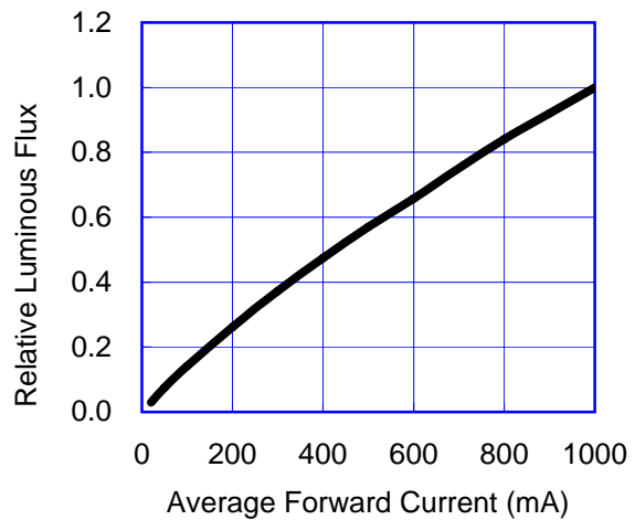
Fig 2. Relative Luminous Flux vs. Forward Current for White and Warm White at T_j=25^\circ\text{C} maintained.
